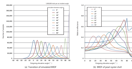
Figure 1: Simulated BRDF and BRDF of pearl oyster shell.
